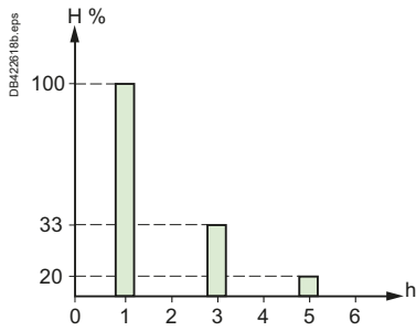
Fig. M9 Harmonic spectrum for a rectangular signal U(t)
