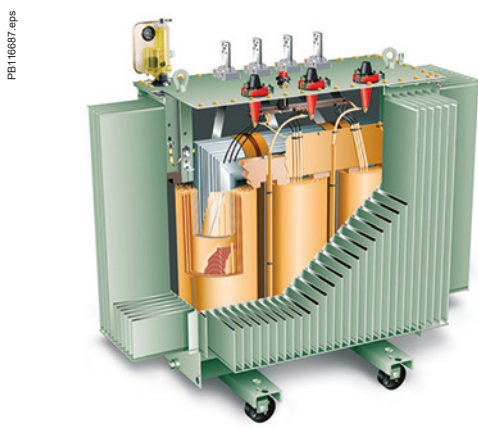
Fig. B17 Integral filled transformer
