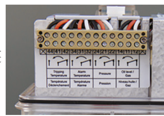
(b) Contacts of the DGPT (cover removed)
