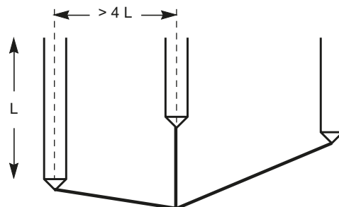
Fig. E21 Earthing rods connected in parallel
