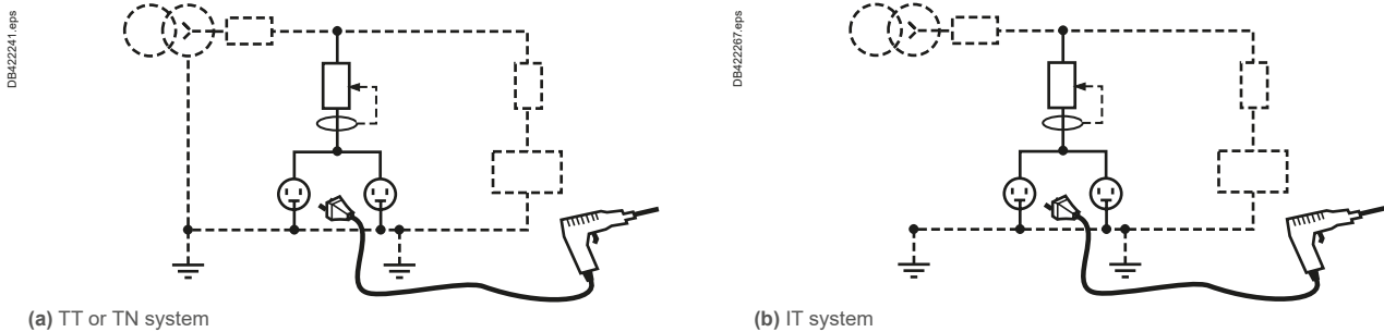
Fig. F10 Circuit supplying socket-outlets
