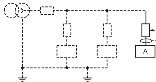
Fig. F17 Unearthed exposed conductive parts (A)
