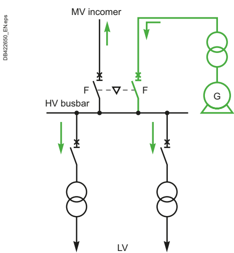
Fig. N13 Energy transfer direction – Generator Set as a generator
