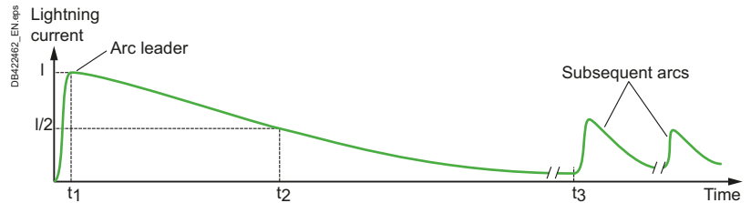
Fig. J4 Example of lightning current
