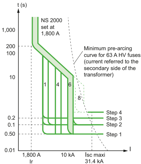
Fig. H57 Curves of MV fuses and LV circuit breaker
