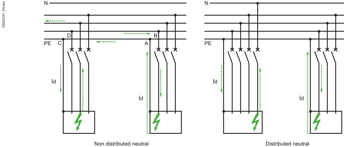
Fig. F39 Calculation of L_{max} for an IT-earthed system, showing fault-current path for a double-fault condition
