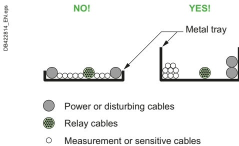
Fig. R48 Cable distribution in cable trays
