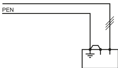
Fig. G56 Direct connection of the PEN conductor to the earth terminal of an appliance
