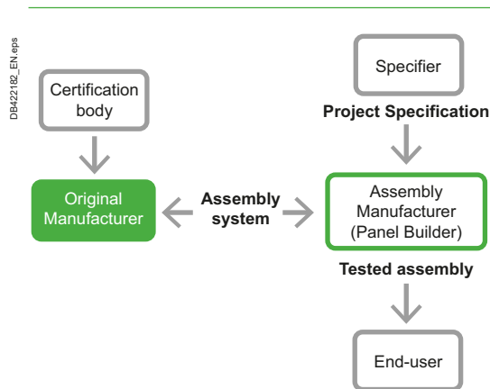
Fig. E33 Main actors and responsibilities, as defined by the IEC 61439-1&2 standard
