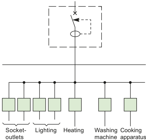
Fig. Q10 Circuit division according to application
