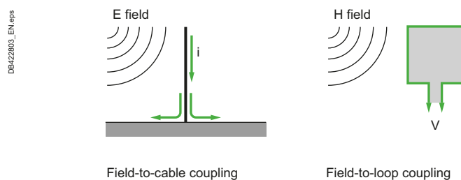
Fig. R37 Definition of radiated coupling
