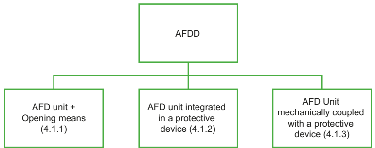
Fig. F90 Methods of construction of Arc fault detection devices
